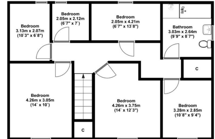
First Floor Approx 89.00 Sq meters (957.00 Sq feet).
