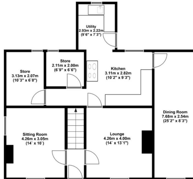
Ground Floor Approx 95.00 Sq meters (1023.00 Sq feet).
